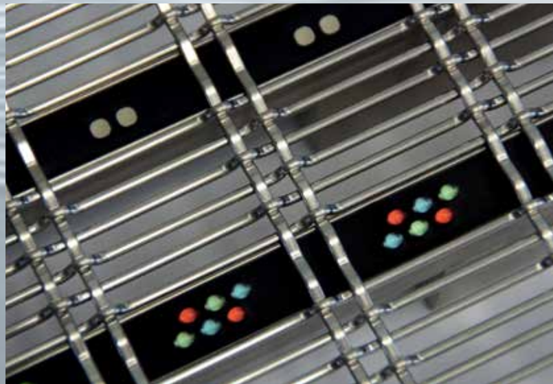
Close-Up: IMAGIC WEAVE® HE (upper) and HO (lower) LED technology.
